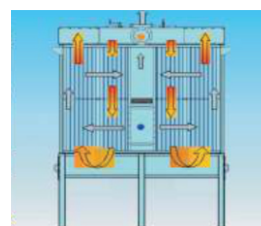
APH - air and flue gas circuit
